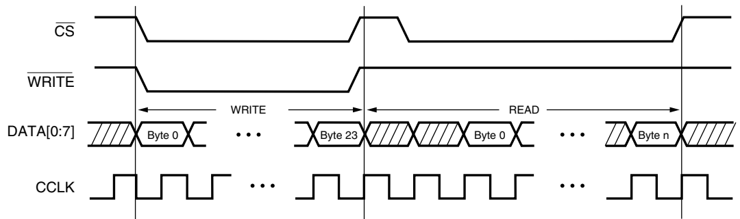
Figure 15: Readback Clocking Sequence
