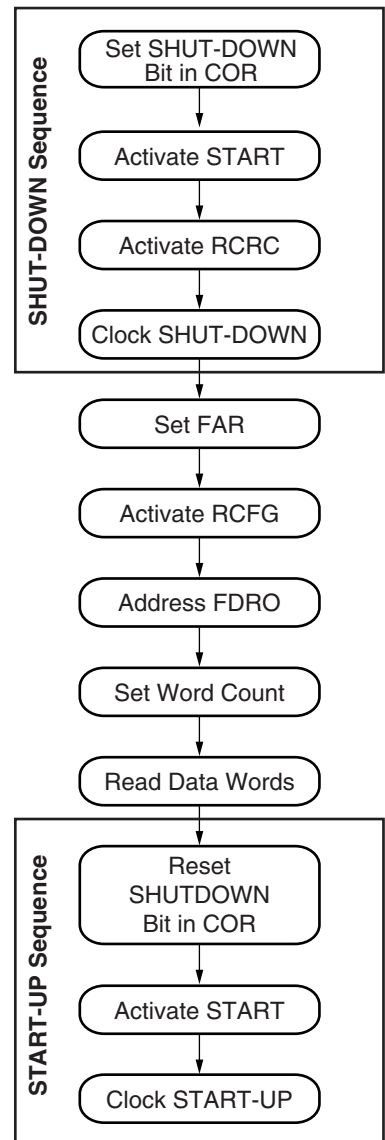
Figure 21: Block RAM Readback Operation Flow
